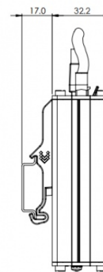
Mounting space requirements
